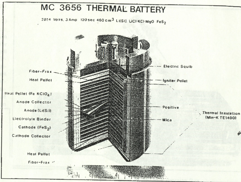
Figure 22. MC3656 Main Battery
